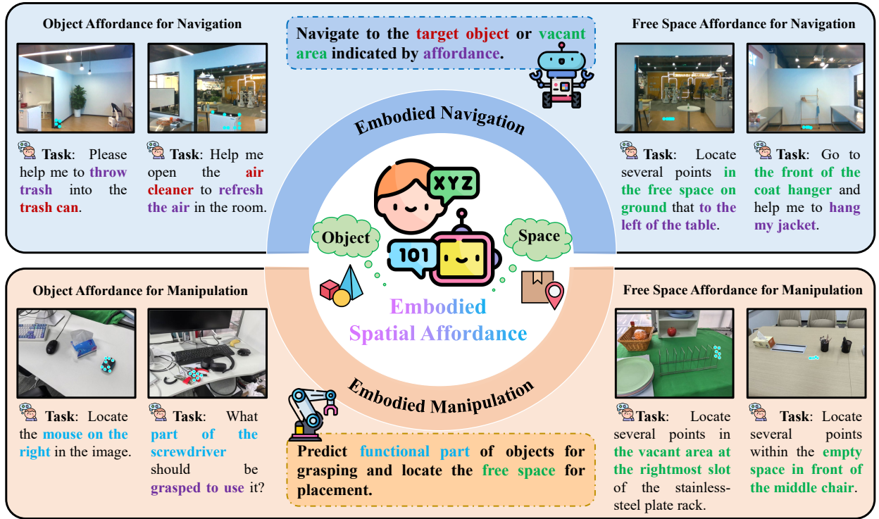
Fig. 1: Overview of the Embodied Spatial Affordance (ESA) dataset. The dataset is categorized into object affordances and free space affordances, supporting both navigation and manipulation tasks. In navigation tasks, the agent must reach a target object or a designated empty area; in manipulation tasks, the agent learns to identify functional parts for grasping and suitable spaces for placement. The ESA dataset integrates spatial reasoning with affordance understanding in an embodied context.
