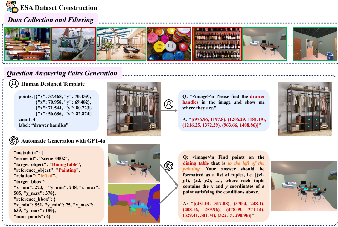
Fig. 2: Pipeline for constructing the ESA dataset. We begin by excluding images with densely repeated objects to ensure quality. Next, we generate question-answering pairs using either human-designed templates or the GPT-4o model [36], facilitating diverse and contextually relevant interactions.
