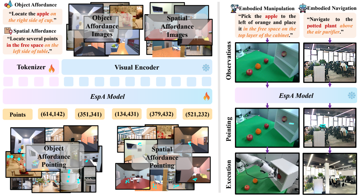
Fig. 3: Framework of EspA. We fine-tune a multimodal language model on the ESA dataset to enhance object and free space affordance capabilities. For downstream embodied navigation and manipulation tasks, we integrate depth images to convert 2D points representing affordances into 3D coordinates, which are then used as target positions for navigation and manipulation.
