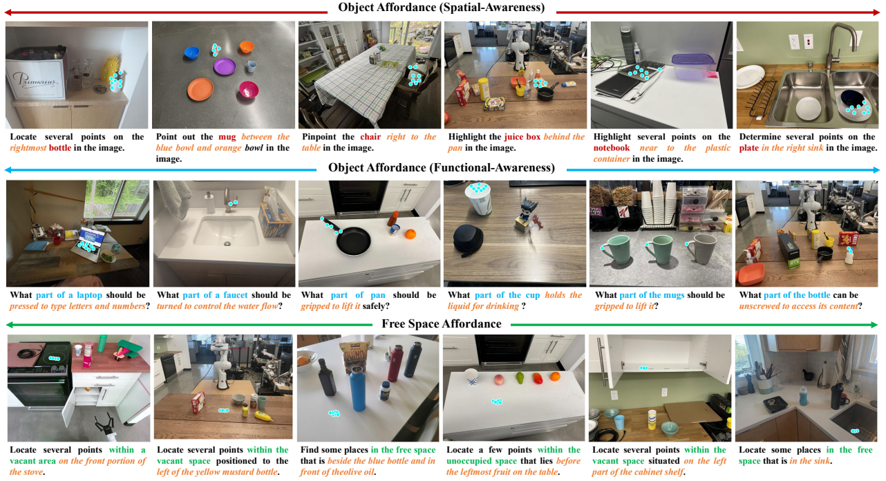
Fig. 6: Qualitative results of EspA model, where cyan points indicate the object and free space affordances.
